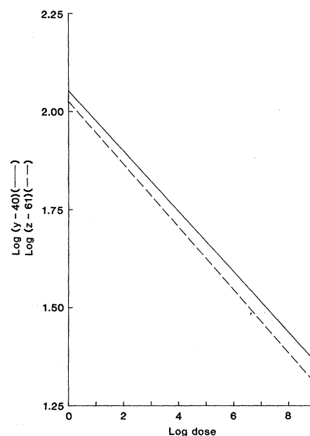
Fig. 2. Assay of the scrapie agent by measurements of the incubation time interval. The intervals from inoculation to onset of illness ( \bar{y} ) and to death ( \bar{z} ) are plotted as a function of the injected dose. Equations were written to describe these linear functions which relate the titer of the inoculum to the time intervals both from inoculation to onset of illness (Eq. 1) and from inoculation to death (Eq. 2):
