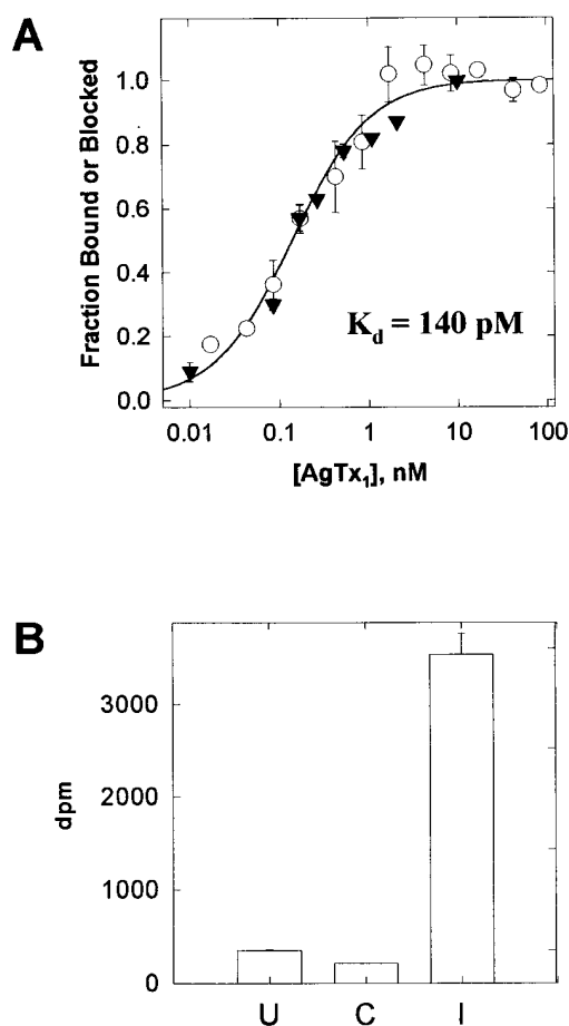
Figure 2. Characterization of [^3\text{H}]\text{NEM} -Conjugated \text{AgTx}_1\text{D20C}
