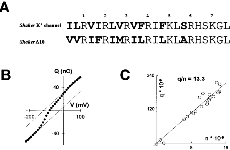
Figure 6. Contribution of Nonbasic Residues in the S4 Segment to Gating Charge (A) The amino acid sequence of the S4 segment in the Shaker K + channel and the Shaker Δ10 mutant channel. All basic amino acid residues are numbered. Mutated nonbasic residues are bold-faced. (B) Q-V plots of repolarization-induced currents for an oocyte. (C) Correlation plots mapping total gating charge (q) in electron charge units as a function of total channel number (n) (n = 21). Channel number was normalized (see text). The line corresponds to a linear regression fit of the data. The gating charge of Shaker Δ10 is not significantly different from that of the wild-type channel.
