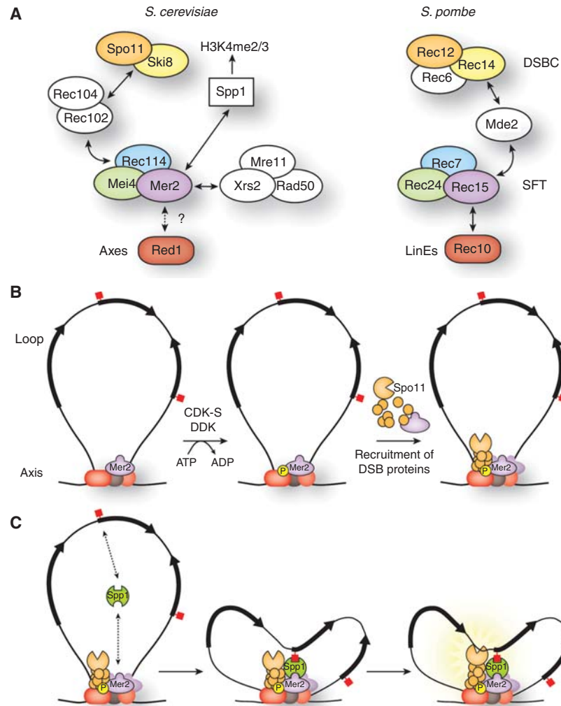
Figure 3. Interaction maps of DSB proteins in S. cerevisiae and S. pombe , and models for roles of DSB proteins in S. cerevisiae . (A) In S. cerevisiae (left), the 10 proteins required for DSB formation form four interacting subcomplexes (see text for details). Mer2 also interacts with Spp1, which recognizes and binds to H3K4me2/me3 marks on chromatin loops. Mer2 and other DSB proteins localize to the chromosome axes, but it is not known whether this is via interaction with the axial element protein Red1 (dashed arrows and question mark), analogous to the interaction of their homologous proteins in S. pombe . In S. pombe (right), the seven proteins required for DSB formation form two subcomplexes (DSBC and SFT) that interact via Mde2. Rec15 interacts with Rec10, a component of linear elements (LinEs) similar to axial elements in S. cerevisiae . Homologous proteins are shown in the same color for the two species; proteins with no known homologs in the other species are shown in white (except for Spp1, whose homolog in S. pombe is not shown, and whose role in DSB formation is not known). (B) Model for DSB regulation via Mer2 phosphorylation (based on data in Henderson et al. 2006; Sasanuma et al. 2008; Wan et al. 2008; Panizza et al. 2011). Mer2 phosphorylation by the replication-associated kinases CDK-S and DDK leads to recruitment of DSB proteins that directly interact with Mer2 (Rec114, Mei4, Xrs2), and perhaps subsequently also other DSB proteins (Rec102, Rec104, Ski8, Spo11, Mre11, and Rad50). Mer2 (purple) is localized at chromosome axes, along with axial element proteins Red1, Hop1, and cohesin Rec8 (red and gray ovals), but is further enriched at axes on phosphorylation by CDK-S. CDK-S primes Mer2 for further phosphorylation by DDK. Arrows on the chromatin loop represent gene open reading frames. Red squares represent H3K4me3 marks. Only one sister chromatid is shown for clarity. (C) Model integrating DSB formation with loop-axis chromosome structure (based on data in Acquaviva et al. 2012; Sommermeyer et al. 2013). Axis-associated Mer2 interacts with Spp1, which binds H3K4me2/me3 marks and thereby tethers a chromatin loop to the axis. The nucleosome-depleted promoter near the tethered loop segment becomes accessible to Spo11, allowing DSB formation. The precise order of events (Mer2 phosphorylation, loop tethering to the axis) is not known. Spp1 interacts with Mer2 independent of Mer2 phosphorylation, so the potential interactions indicated in the left-most panel (H3K4me2/me3–Spp1–Mer2) could also occur in B, but are not shown.
