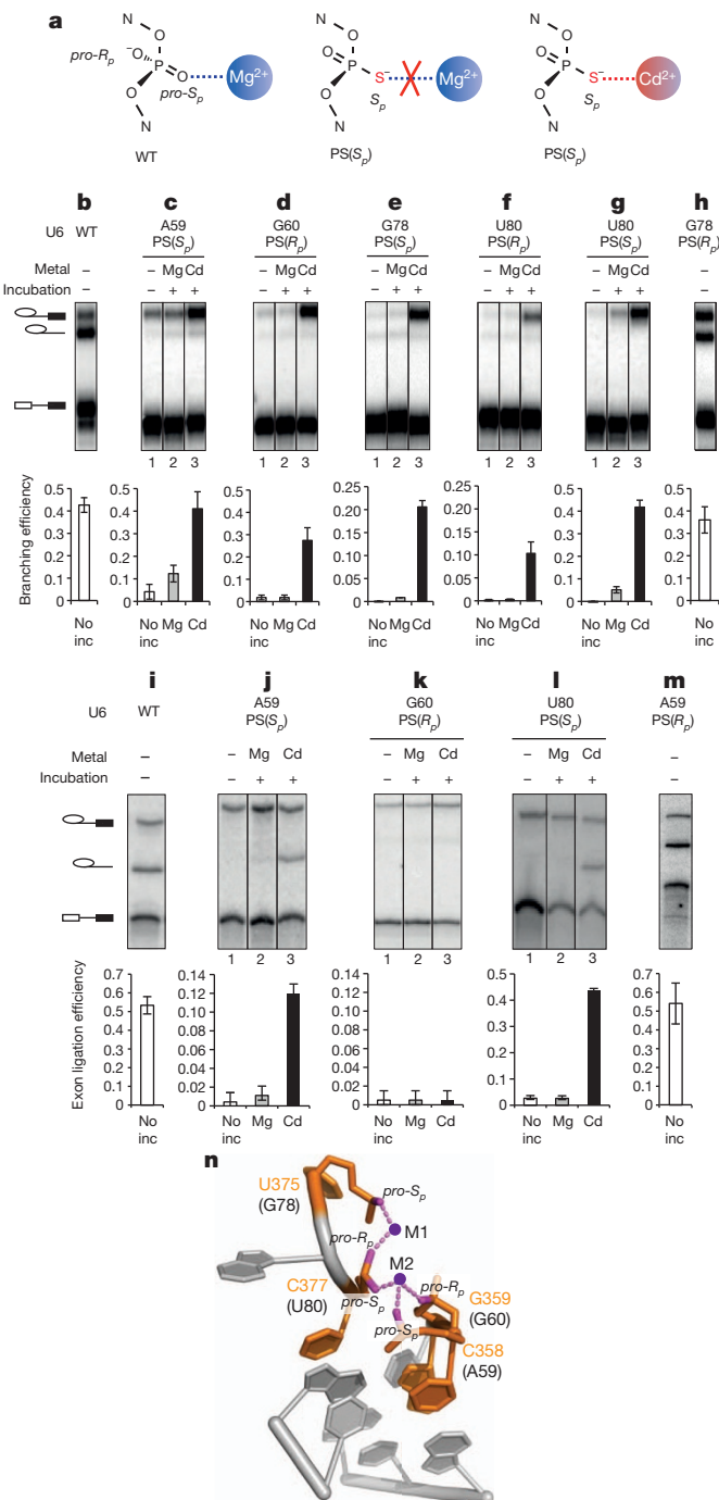
Figure 2 | U6 snRNA positions metals important for both steps of splicing. a , Metal rescue strategy, indicating the non-bridging oxygens that were substituted with sulphur and the consequence of a substitution for binding of Mg 2+ or the thiophilic metal Cd 2+ . b–m , Cd 2+ rescues the branching defects ( b–h ) and exon ligation defects ( i–m ) induced by specific sulphur substitutions. Values represent averages; error bars, s.d. ( n = 3 for b–h ; n = 2 for i–m ); no inc, no incubation. n , Structure of the domain V metal binding core (PDB 3EOH, ref. 26). Residue numbers are shown for the group II intron, with the corresponding U6 residues in parentheses.
